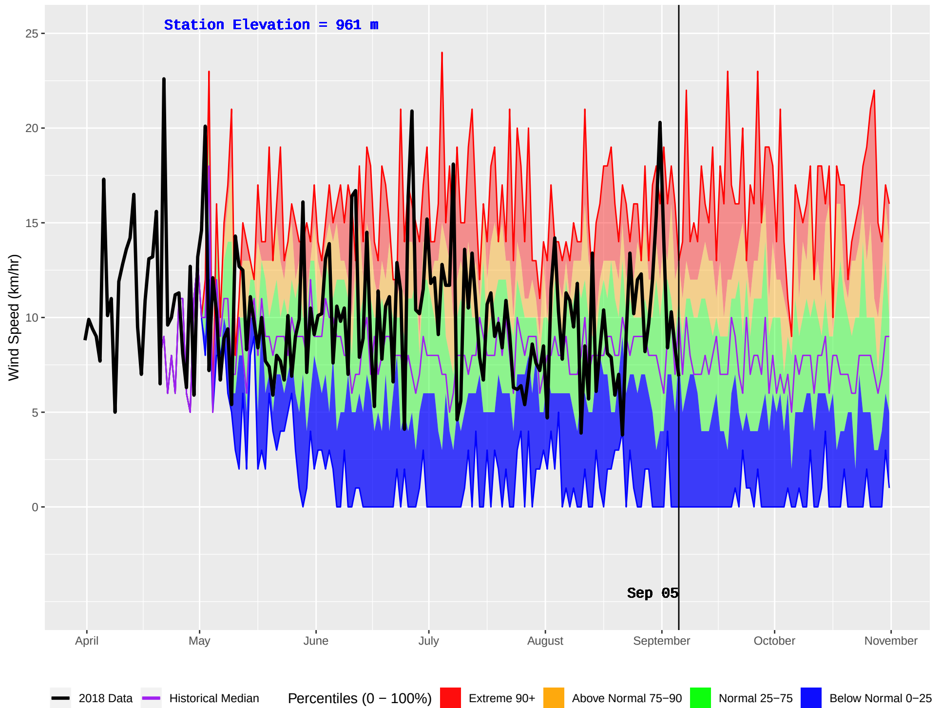
HOLY CROSS 2 (654) : Historical (1998–2016) and Current (2018) Daily Wind Speed
